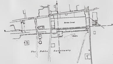
RELATIVE SITE PLAN 480 To show position of Sections Scale of Feet 480
